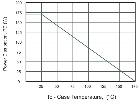
Fig.4 Power Dissipation
